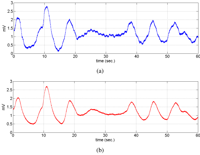
Fig. 5. Typical segment of ECG BW Noise (a) Original (b) Synthetic
