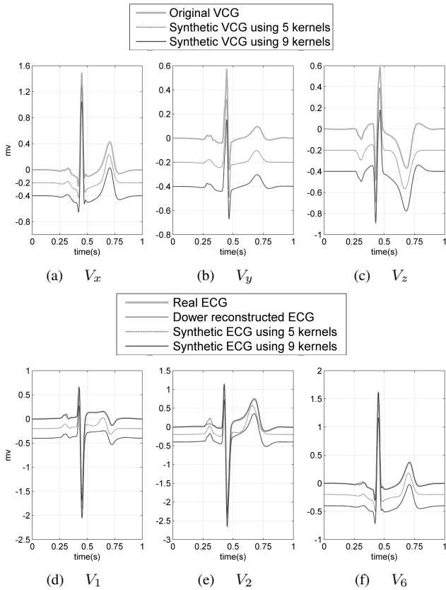
Fig. 7. Original vs. synthetic VCGs and ECGs using 5 and 9 Gaussian functions. For comparison, the ECG reconstructed from the Dower transformation is also depicted in (d)-(f) over the original ECGs. The synthetic VCGs and ECGs have been vertically shifted 0.2mV for better comparison. Refer to text for details.
